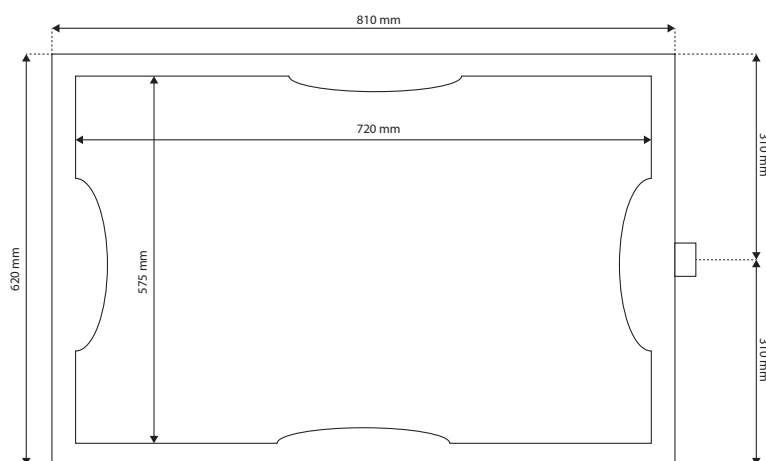
TRIPOND Modulfilter
